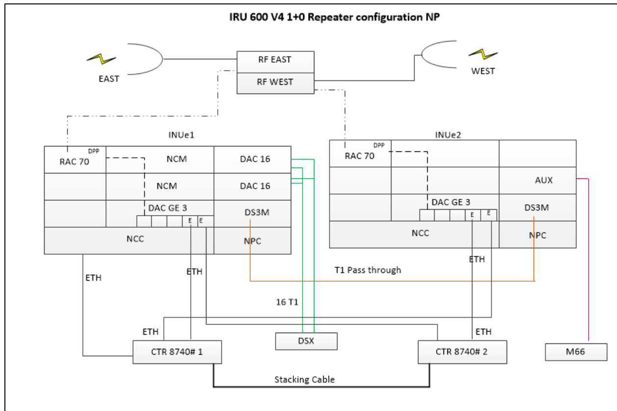
Typical SBD for a loop site facing EAST and WEST
