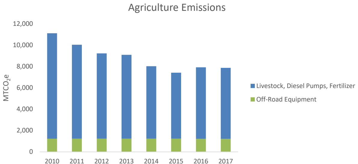
Figure 16. Agricultural GHG emissions in MTCO 2 e from 2010–2017.
