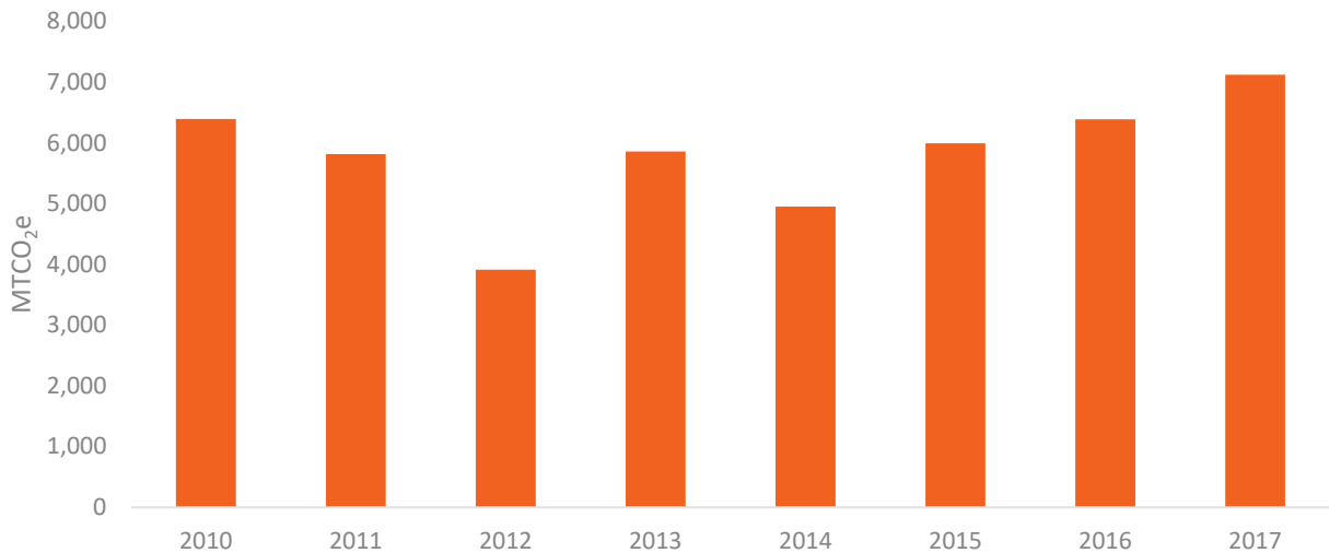
Figure 15. Solid waste GHG emissions in MTCO 2 e from 2010–2017.
