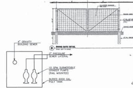
BUILDING WASTEWATER STORAGE AND FLOW EQUALIZATION (ONE PER BUILDING, LOCATED IN UTILITY ROOM)
