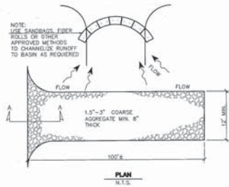
B STABILIZED CONSTRUCTION ENTRANCE DETAIL SCALE: (NOT TO SCALE)
